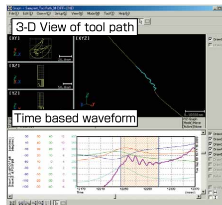
Tool path with time based waveform
